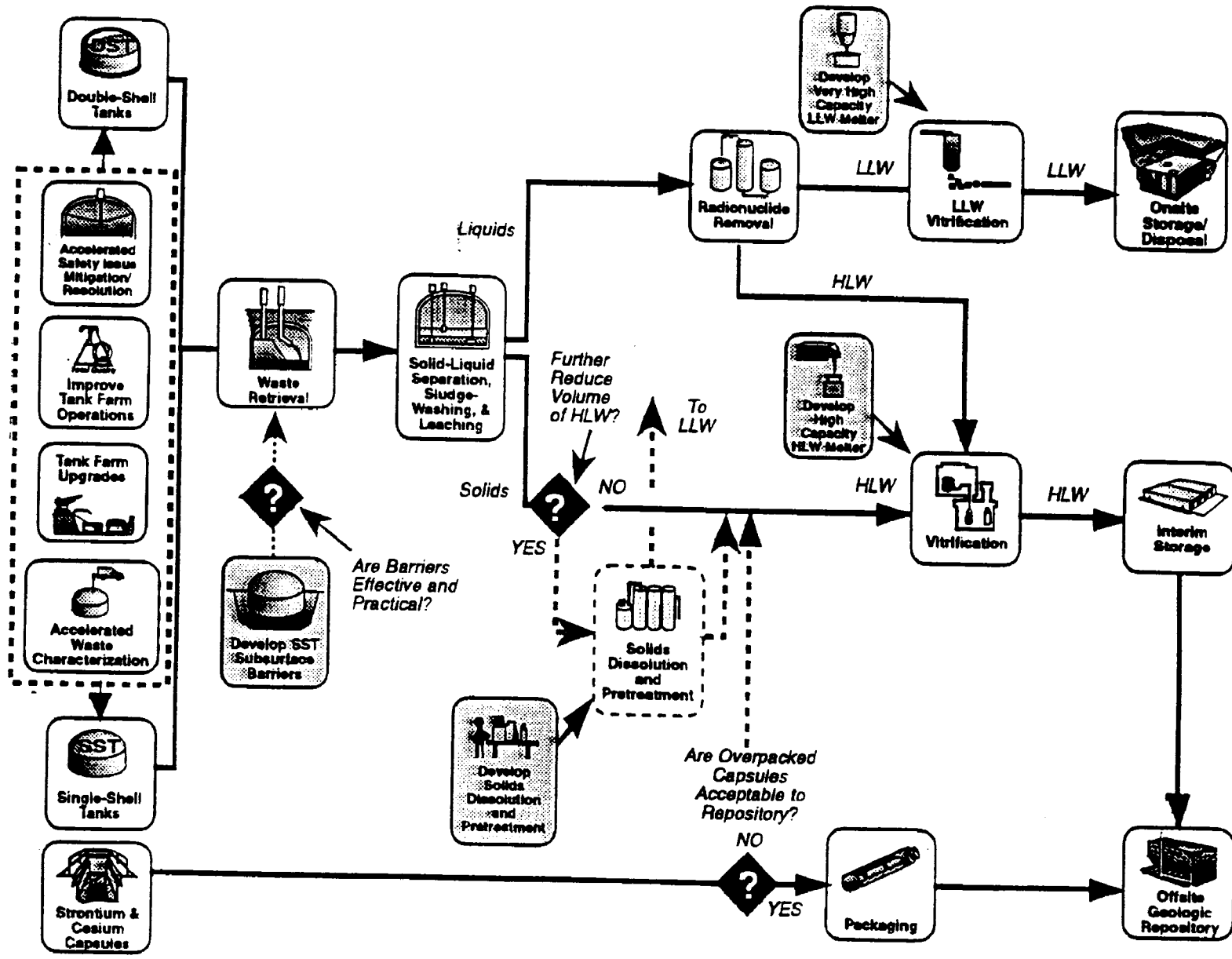
Figure B-1. Proposed Hanford Tank Waste Remediation System.
