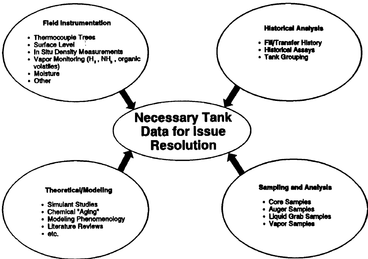
Figure 2. Strategy for Tank Characterization.
